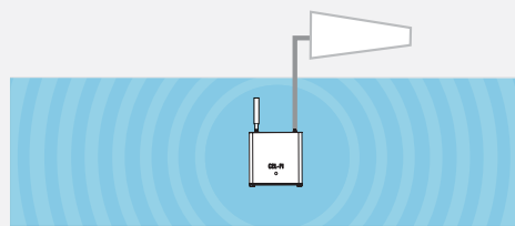
External Donor Antenna
